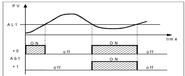
example with absolute low alarm
