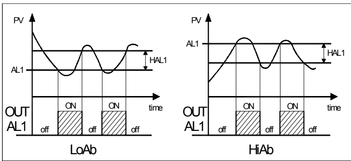
example with absolute low alarm
