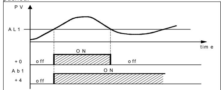
example with absolute high alarm
