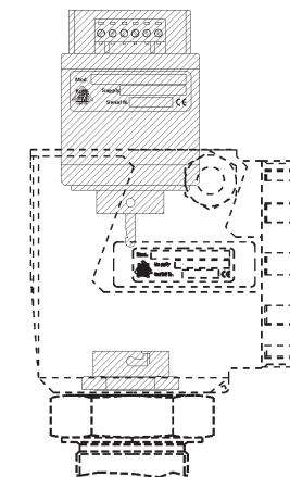
fig.2 SEPARATE-ELECTRODE VERSION DIN-A Double cover PBT + 1,5 coaxcable TC
